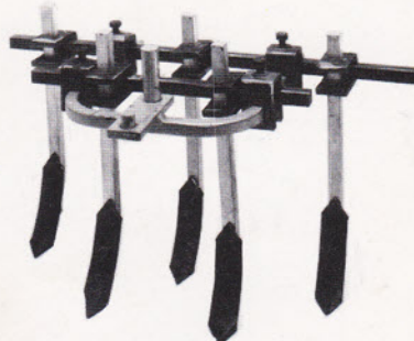
Tool Frame with Cultivating Points and Stalks.
