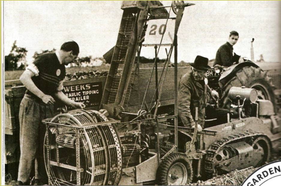
Ransomes M65 with Henderson potato lifter. Photo taken from period advertising literature
