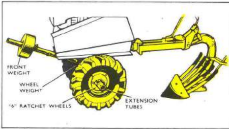
MT 4562 Plough c/w Mounting Bracket MT 3336 Front Weight and Bracket (set) MT 3386 Wheel Weights (pair)
