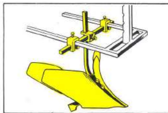
Fitted on MT 2760 MT 2991 Heavy Duty Furrower with MT 3051 Clamp MT 2764 15" Cross Bar MT 2738 Clamps
