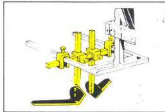
Fitted on MT 2760 MT 2741 Side Hoe – left-hand MT 2746 Side Hoe – right-hand MT 2764 15" Cross Bar MT 2738 Clamps
