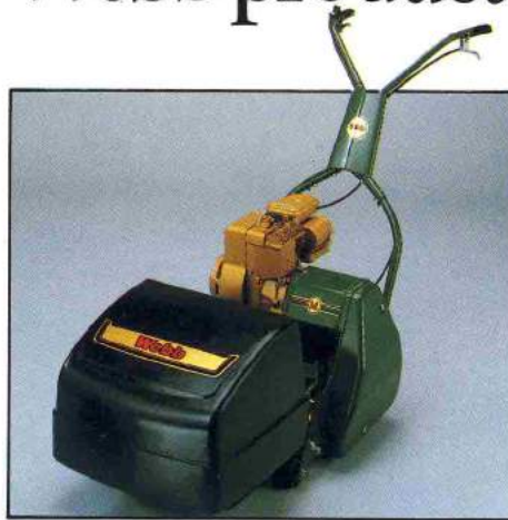
Webb AB 1474 14" Motor Mower with Grassbox Also available as 18" Model No AB 1476.
