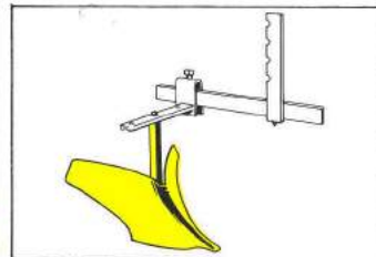
Fitted on MT 1530 - MT 2403 12" Furrower with MT 3051 Clamp
